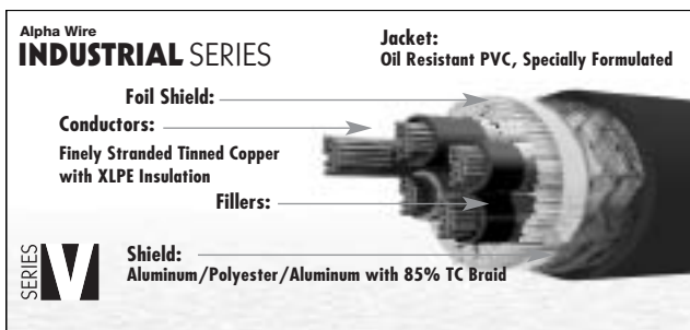
The SERIES V round, symmetrical design offers cable attributes that typical convoluted cables do not.
